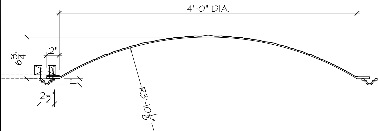
1B DETAIL SECTION SCALE : 1-1/2" = 1'-0"
