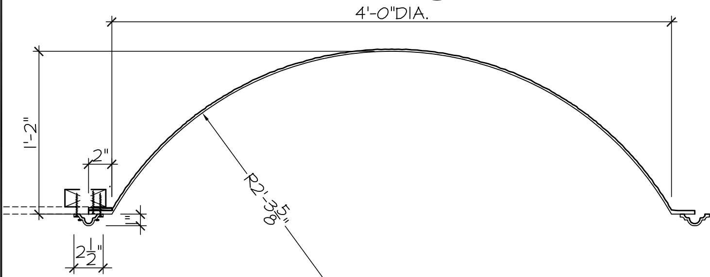
1B DETAIL SECTION SCALE : 1-1/2" = 1'-0"
