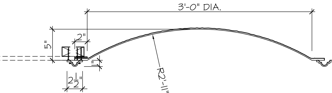
1B DETAIL SECTION SCALE : 1-1/2" = 1'-0"
