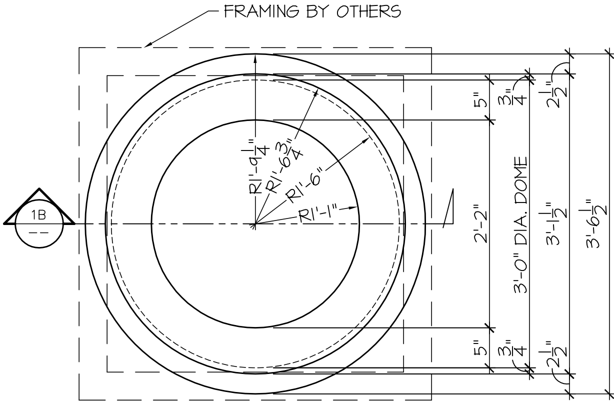
1A REFLECTED PLAN VIEW SCALE : 1" = 1'-0"
