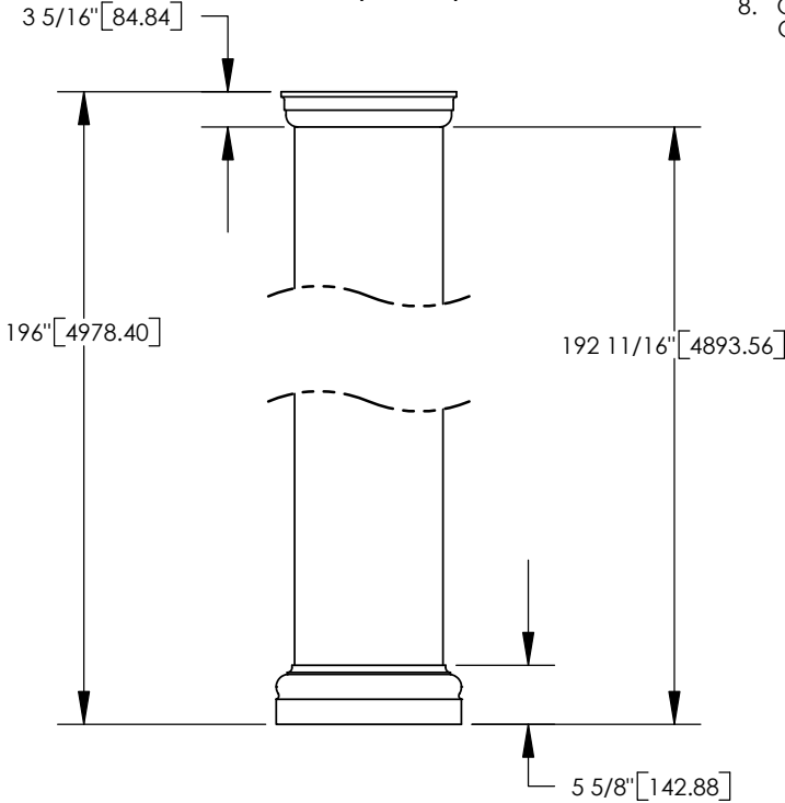
SQUARE TUSCAN 1 3/4" 1 3/4" 14" CAP
