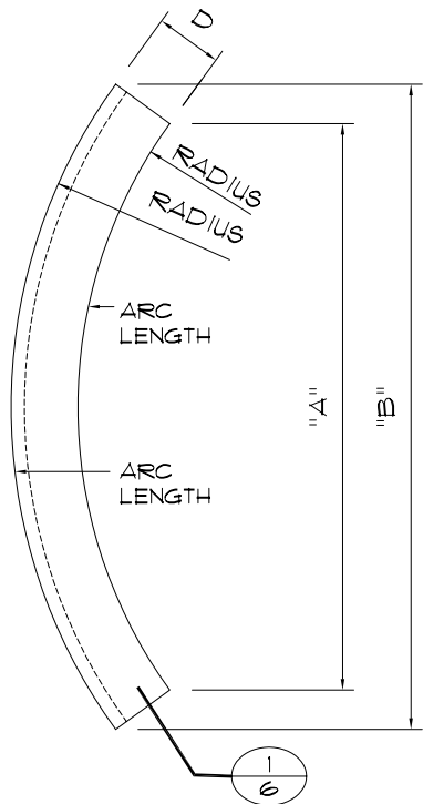
GRG LIGHT SHELF GEOMETRY - PN 02 N.T.S.
