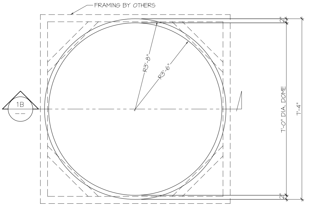
1A REFLECTED PLAN VIEW SCALE : 1/2" = 1'-0"
