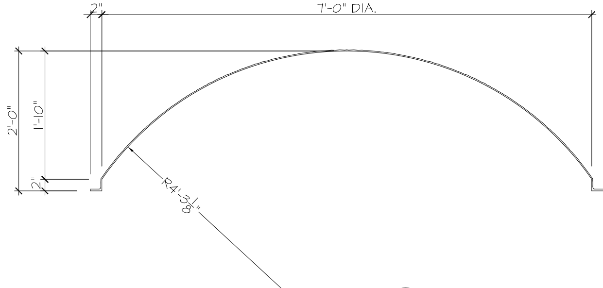
1B DETAIL SECTION SCALE : 3/4" = 1'-0"
