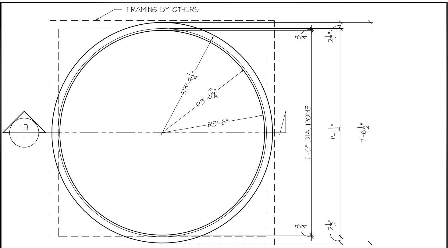
1A REFLECTED PLAN VIEW SCALE : 1/2" = 1'-0"
