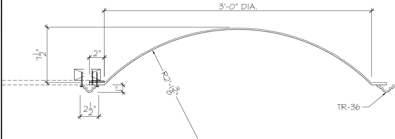
1B DETAIL SECTION SCALE : 1-1/2" = 1'-0"
