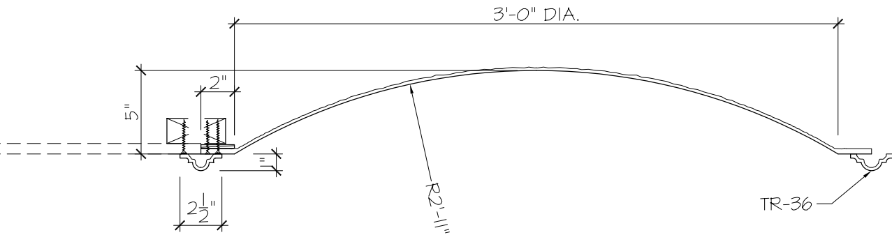
1B DETAIL SECTION SCALE : 1-1/2" = 1'-0"
